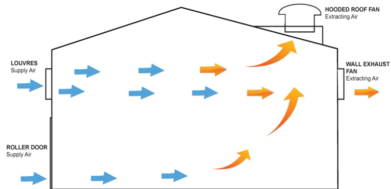
CROSS FLOW VENTILATION
